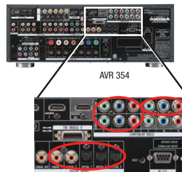
Figure 22 – Connecting a Component-Video-Equipped Disc Player
