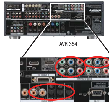
Figure 25 – Connecting a Component-Video-Equipped Recorder
