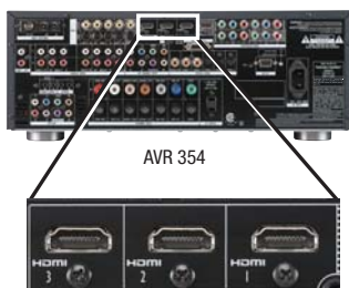
Figure 20 – Connecting an HDMI-Equipped Disc Player
